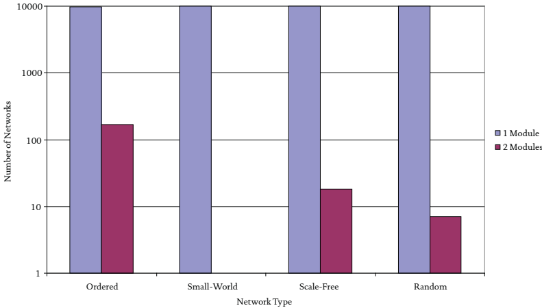
Figure 4 Profile of modular frequency in topologically different Boolean networks comprising fifteen nodes.
