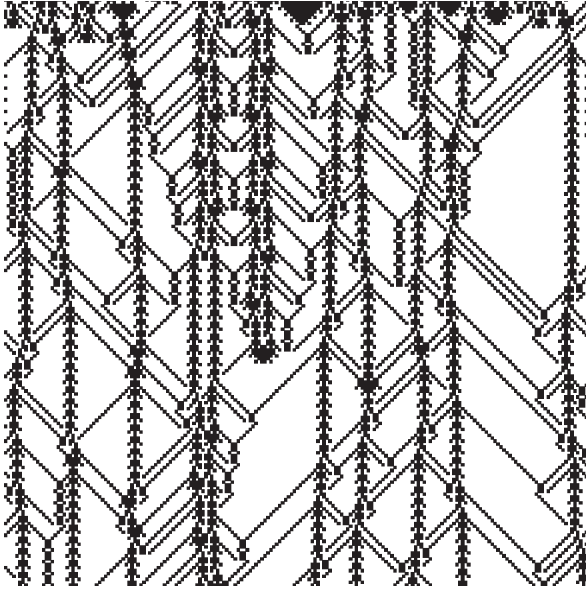
Figure 2 Pattern-basis-filtered CA
