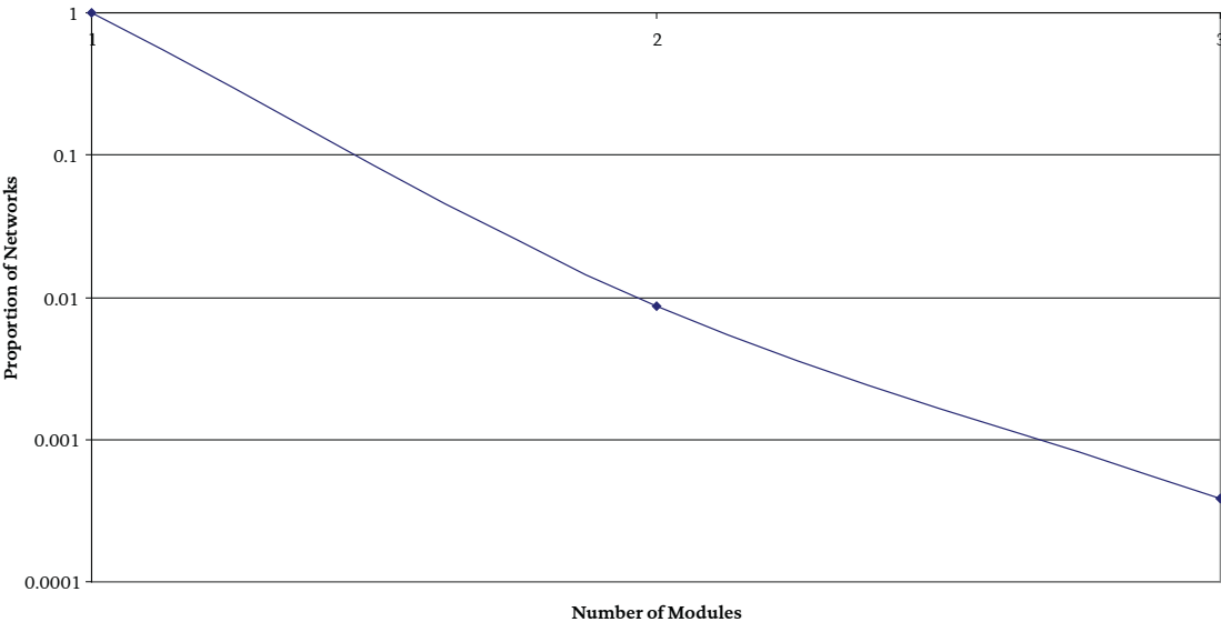
Figure 5 Modular frequency in random Boolean networks comprising twenty nodes (and three connections per node)..
