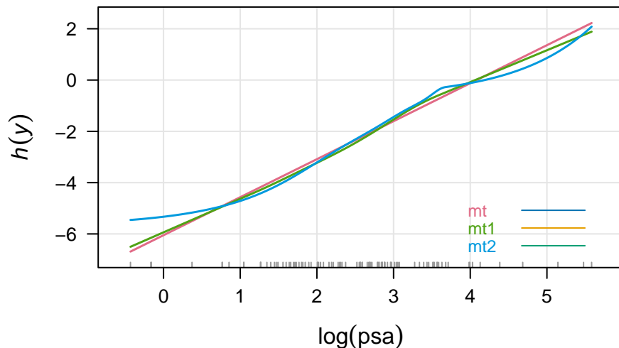
Figure 1: Comparison of different choices for the baseline transformation of the response (prostate specific antigen concentration) in the Prostate data. The original analysis prespecified a log-transformation of the response and then assumed conditional normality on this scale. Hence the baseline transformation of mt is of the form: h(lpsa) = \vartheta_1 + \vartheta_2 \cdot lpsa . Now one can allow a more flexible transformation function in \log(psa) to judge any deviations of h(\log(psa)) from linearity, leading to a baseline transformation in terms of basis functions: a_{Bs,7}(\log(psa))^T \vartheta in mt1 . Lastly, instead of presuming a log-transformation one could estimate the baseline transformation from the raw response ( psa ), i.e. h(psa) = a_{Bs,11}(psa)^T \vartheta in mt2 . In this case, a higher order basis expansion was chosen to account for the skewness of the raw response. Notably, all three baseline transformations are fairly comparable. The basis expansion in psa deviates from being log-linear towards the boundaries of the response's support, as there are only few observations.
